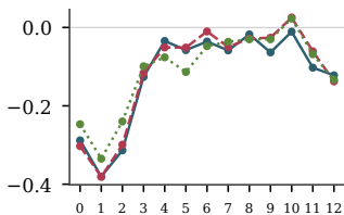
Phrase Role
