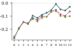
Arc Direction
